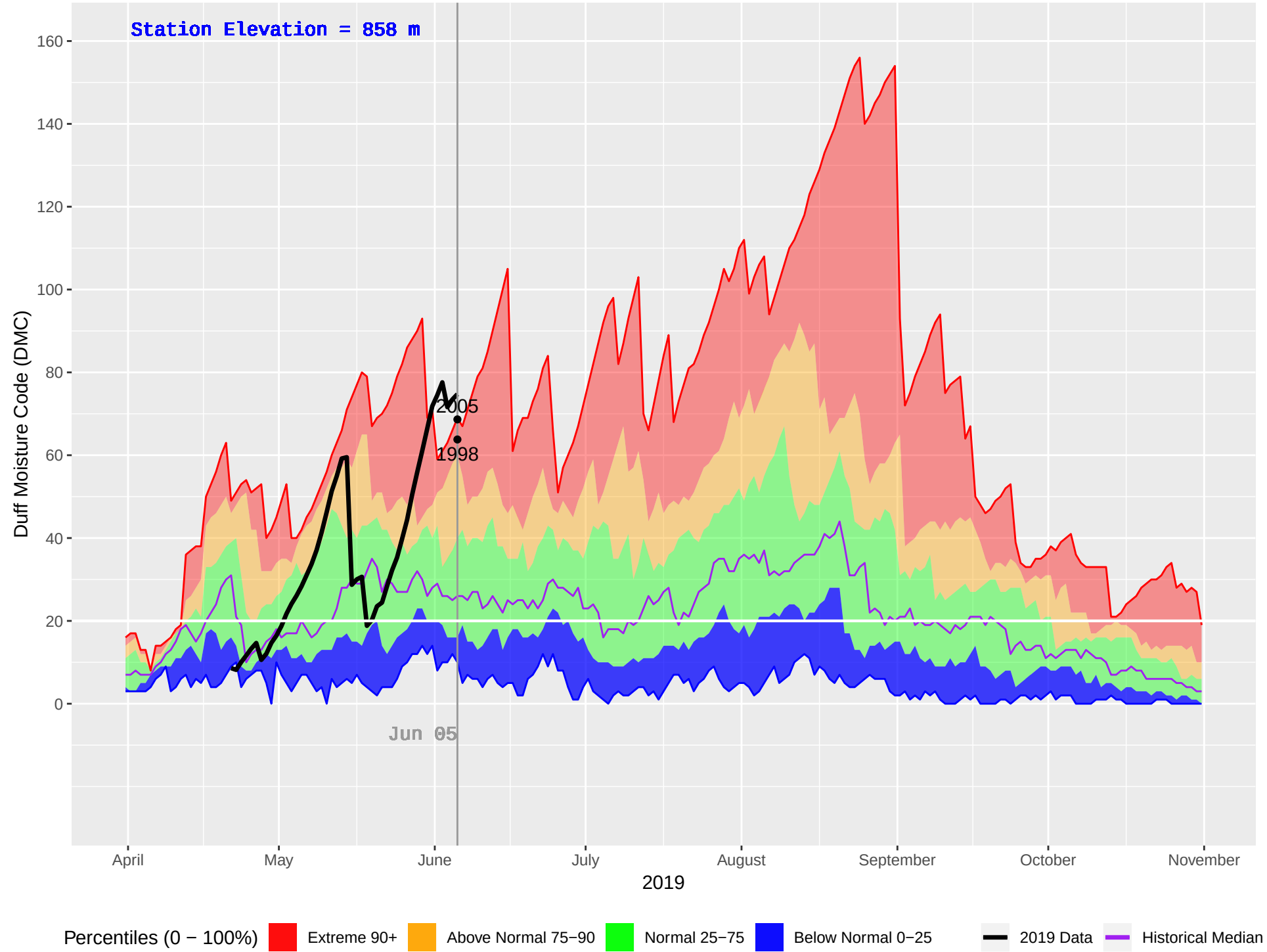
BEDNESTI (175) : Historical (1993–2018), Current (2019) Daily Duff Moisture Code (DMC)
