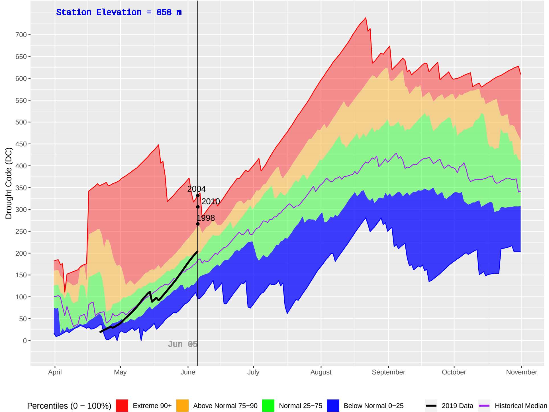
BEDNESTI (175) : Historical (1993–2018) and Current (2019) Daily Drought Code (DC)
