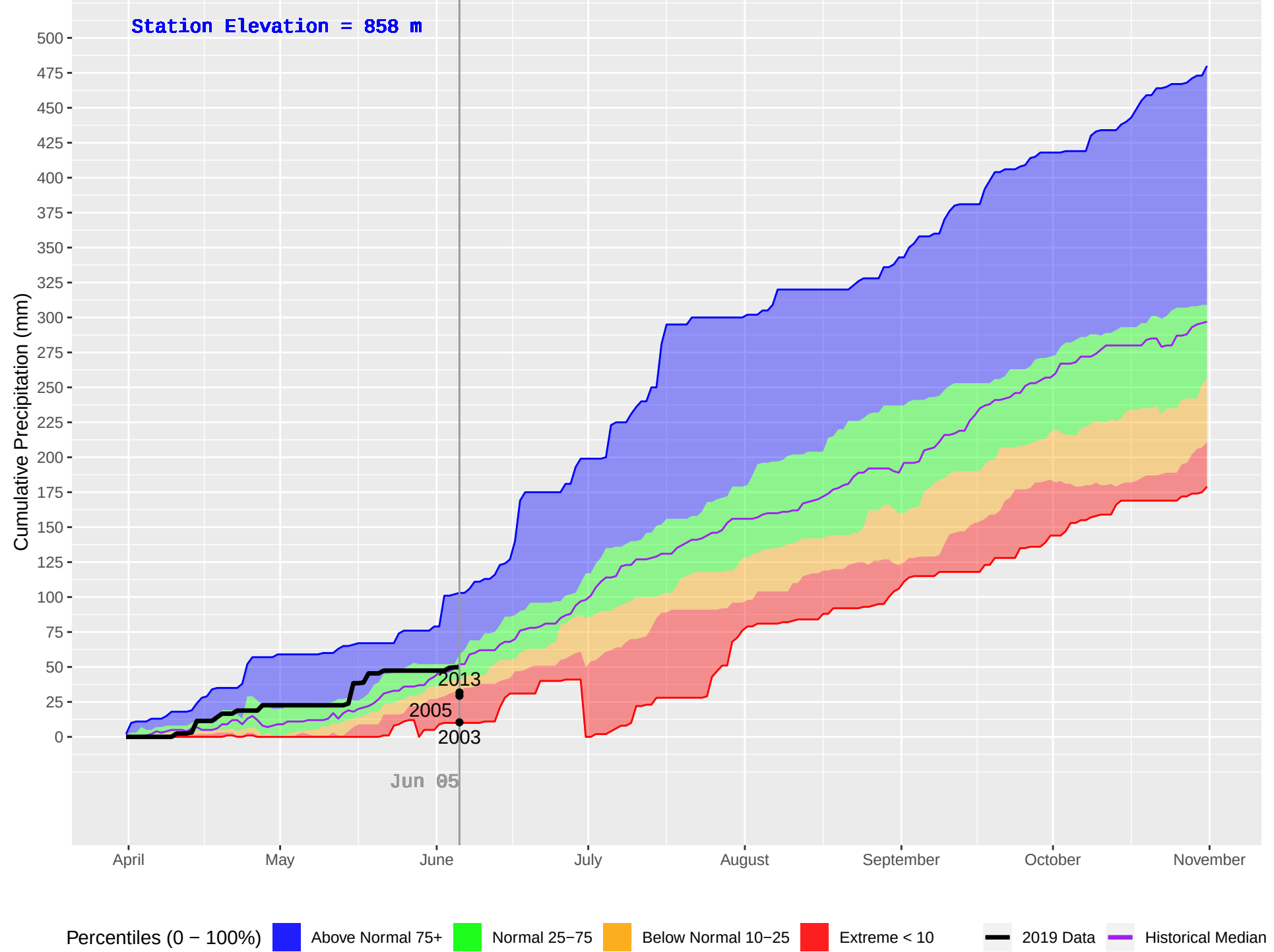
BEDNESTI (175) : Historical (1993–2018), Current (2019) Daily Cumulative Precipitation
