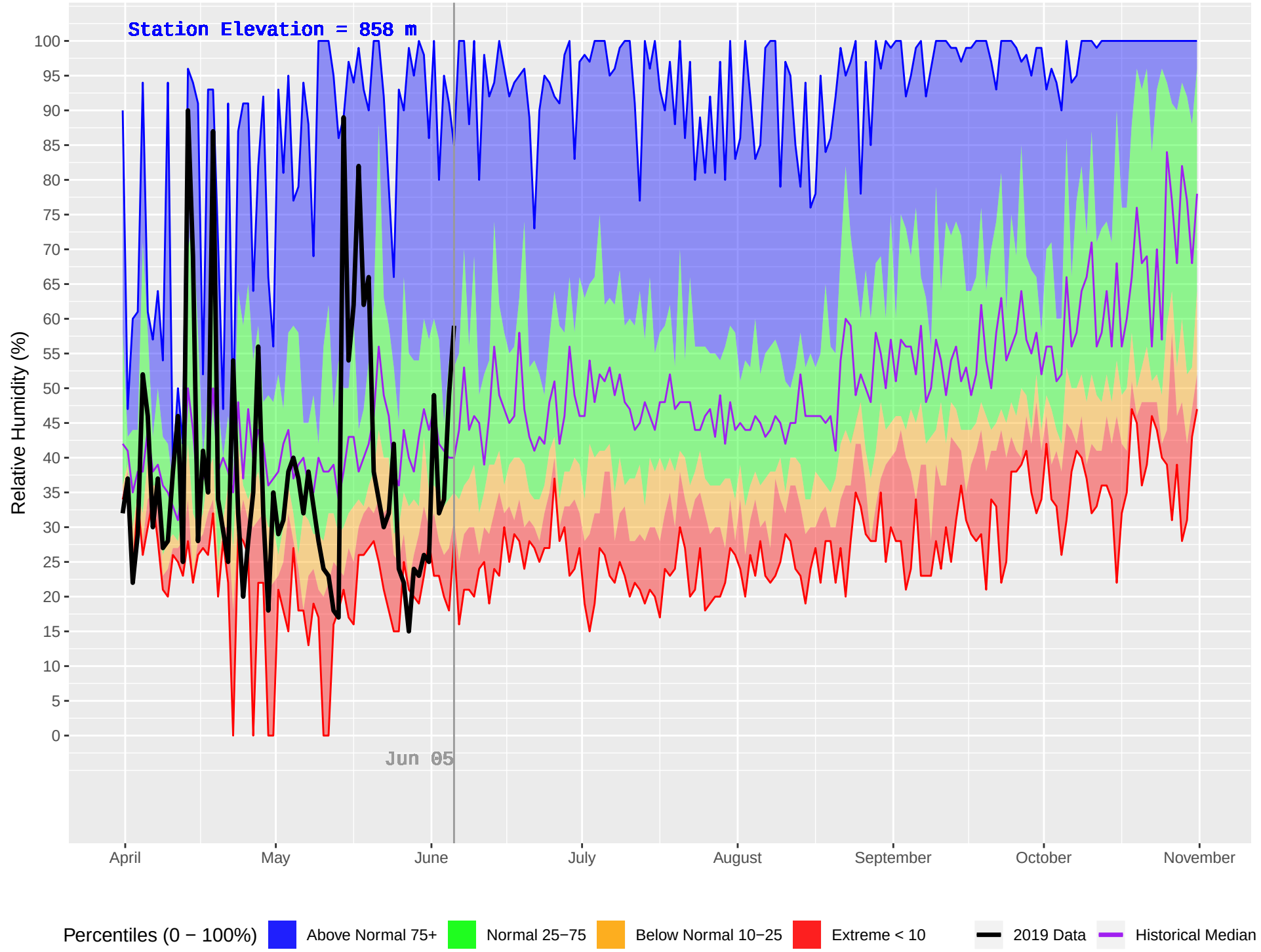
BEDNESTI (175) : Historical (1993–2018) and Current (2019) Daily Relative Humidity
