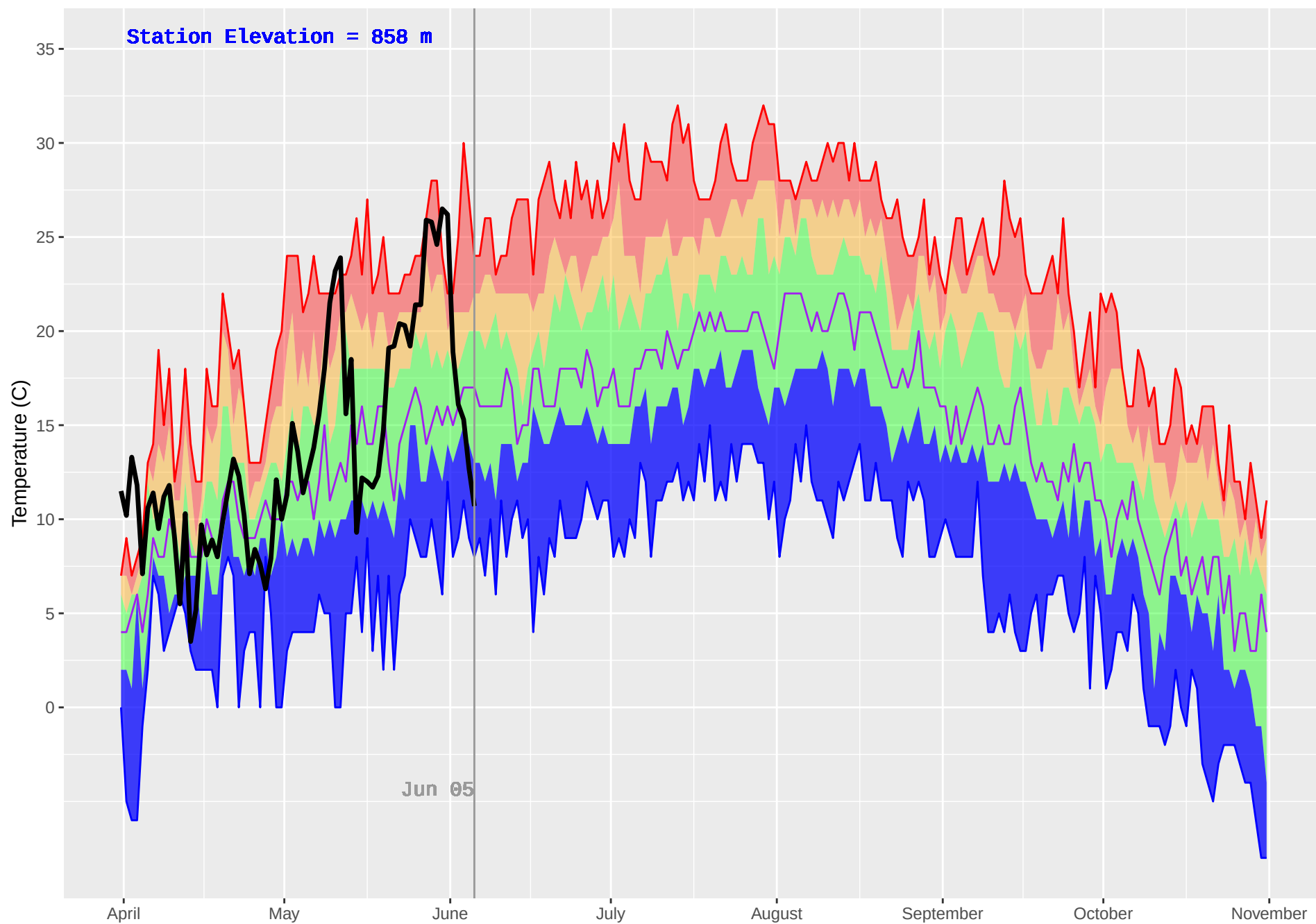
BEDNESTI (175) : Historical (1993–2018) and Current (2019) Daily Temperature
