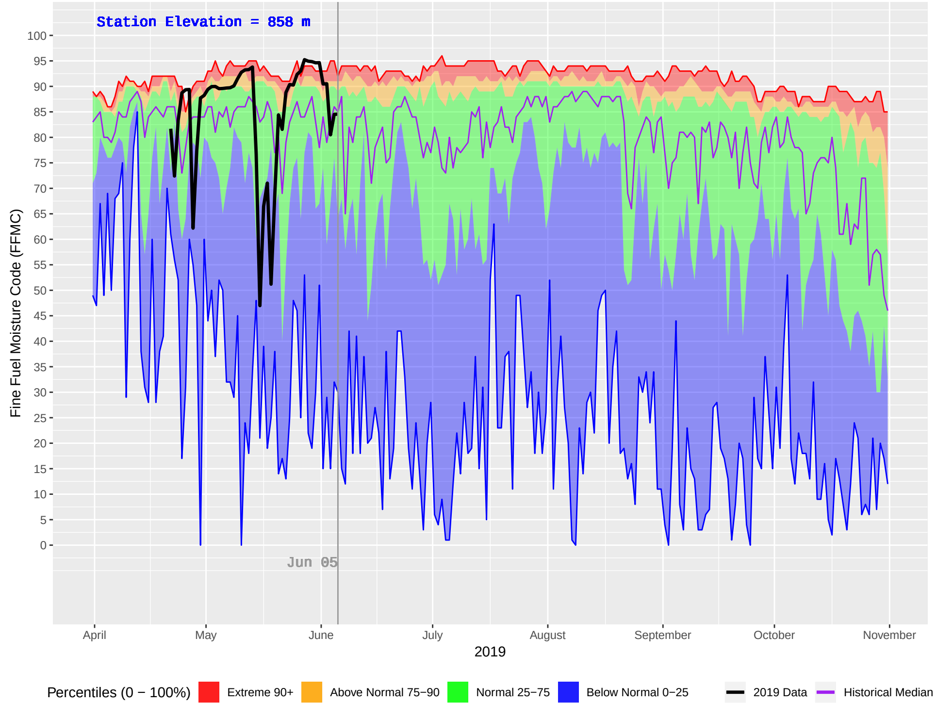
BEDNESTI (175) : Historical (1993–2018) and Current (2019) Daily Fine Fuel Moisture Code (FFMC)
