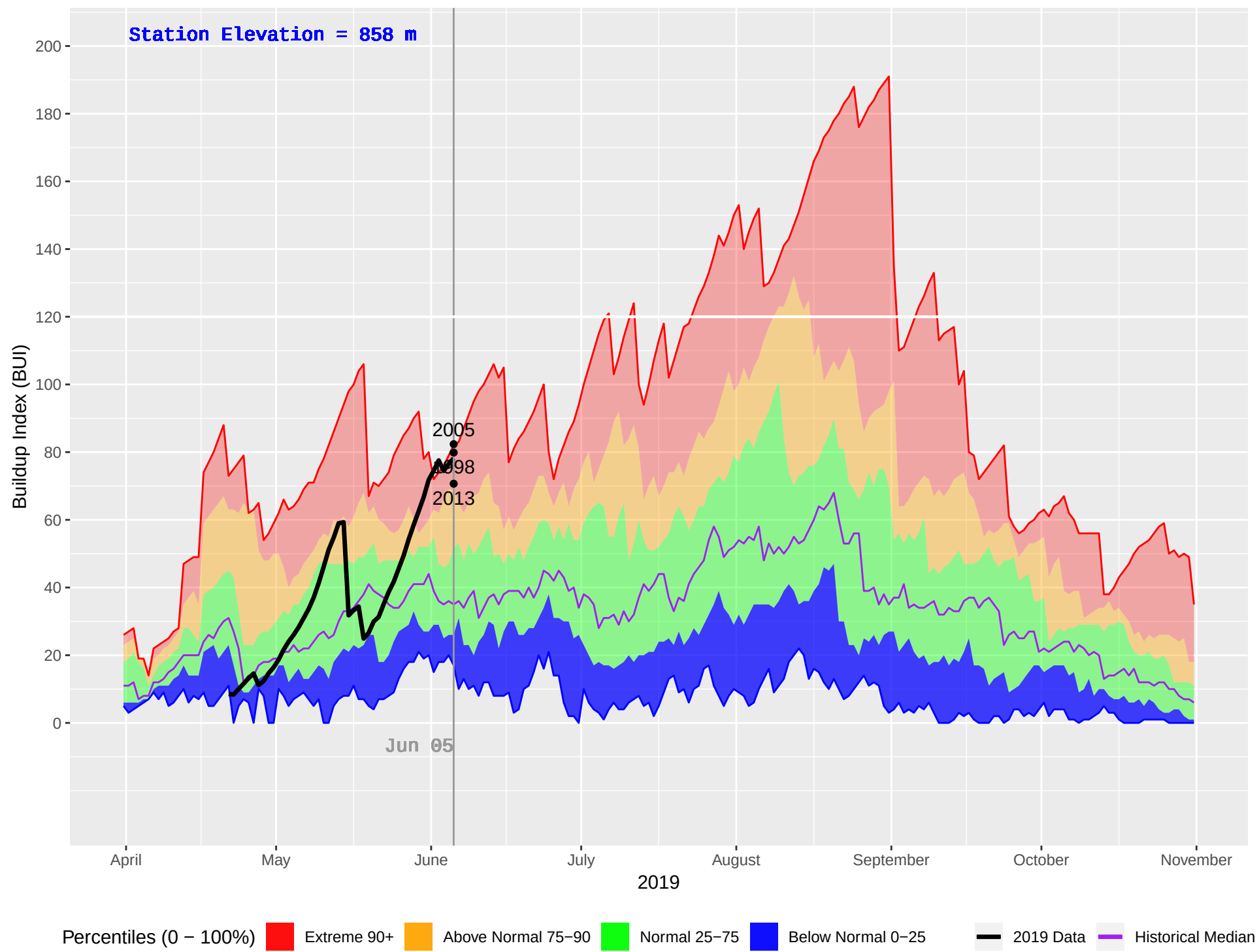
BEDNESTI (175) : Historical (1993–2018), Current (2019) Daily Buildup Index (BUI)
